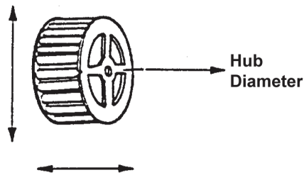
Single Inlet Wheel (Air drawn in from one side only.)
